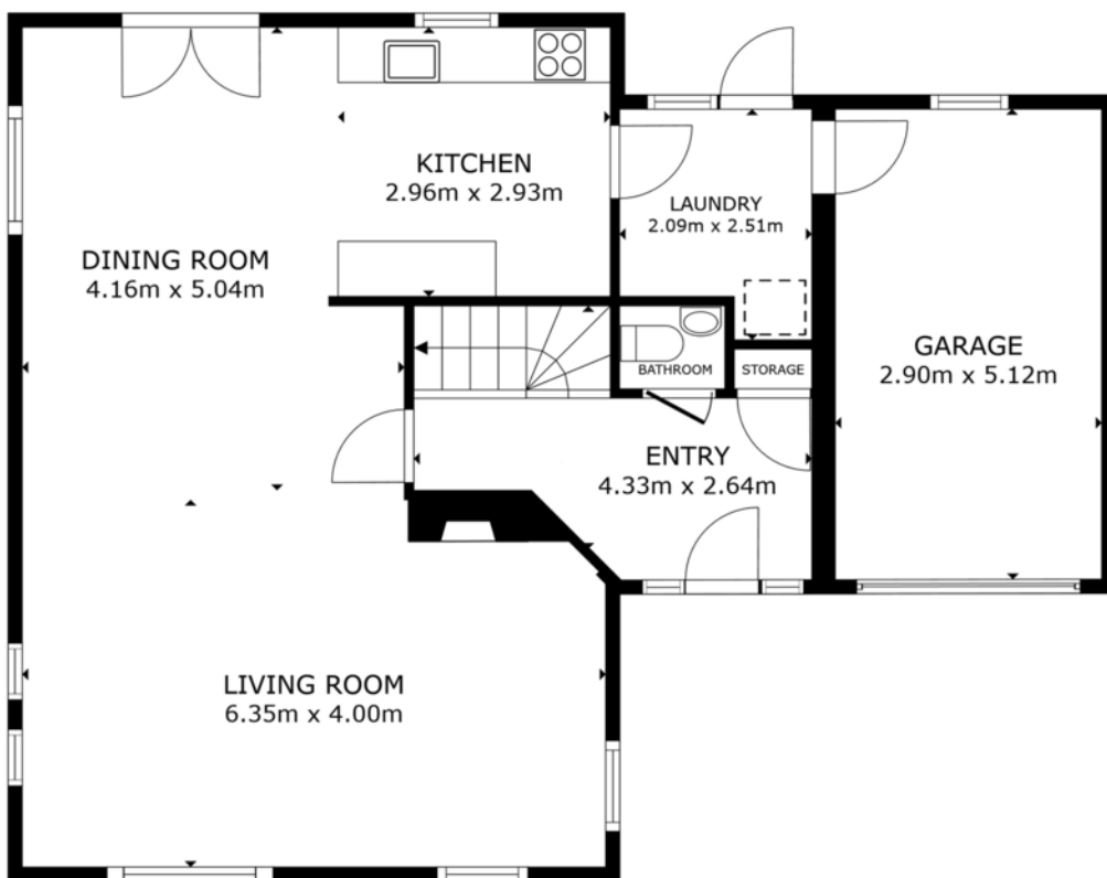
FLOOR 1
