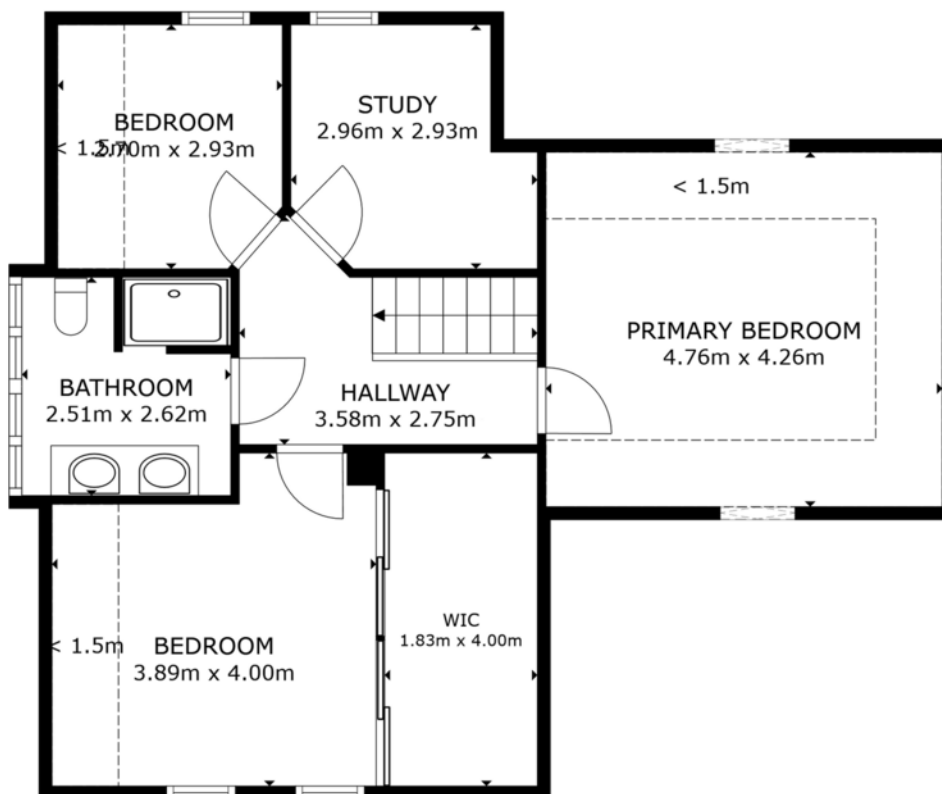
FLOOR 2
