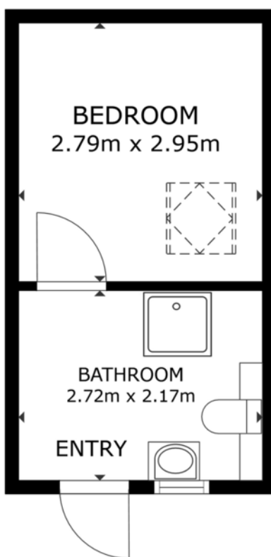
FLOOR PLAN
