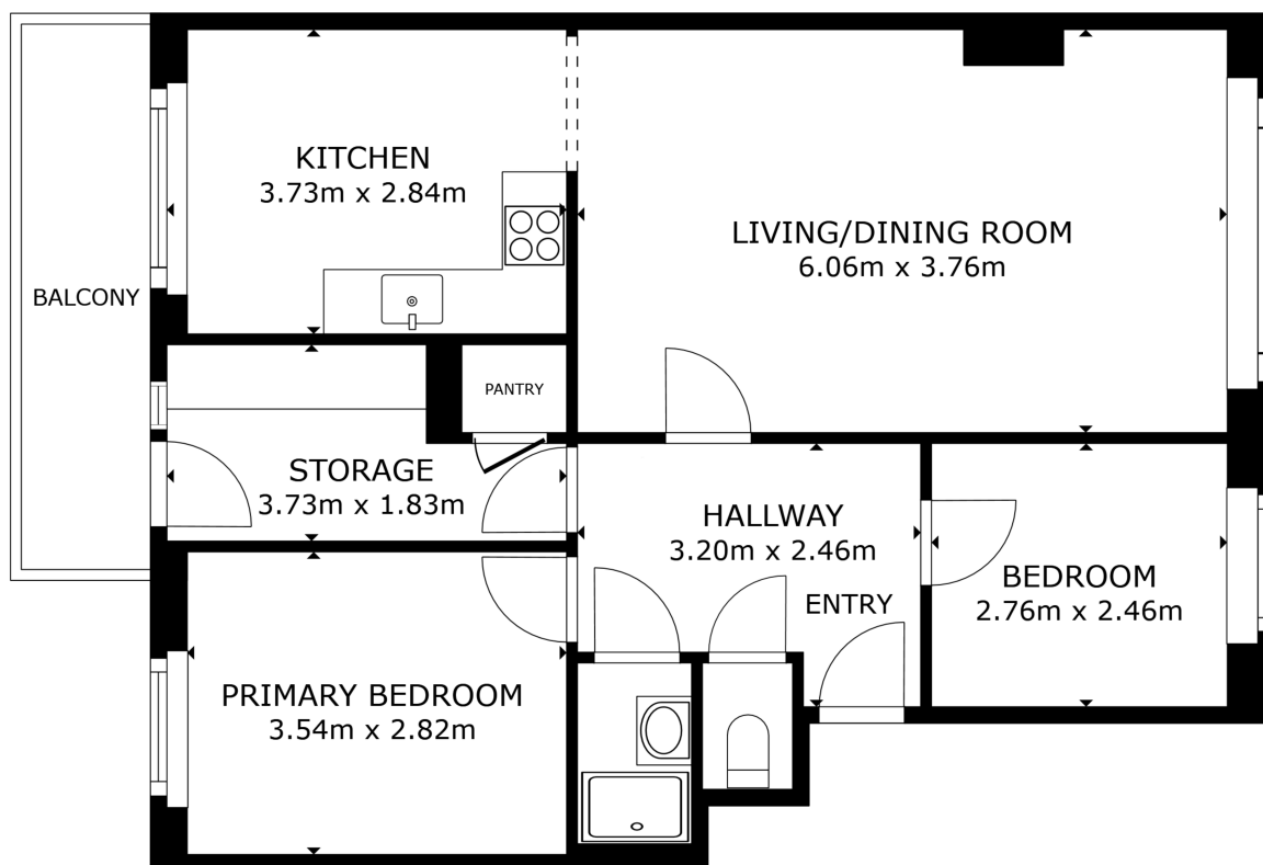
FLOOR PLAN
